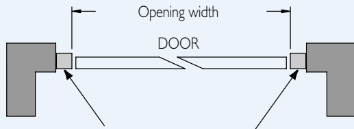
Fitting to timber frame, within the brickwork aperture
