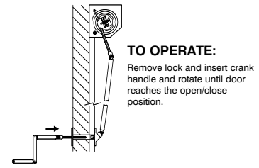
Internally installed shutter with external manual override
