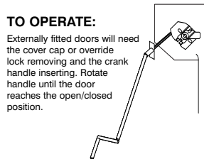
Externally installed shutter with external manual override
