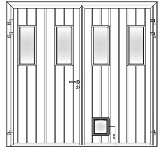
Standard Ribbed Vertical. 50/50 Rectangle windows. Catflap.
