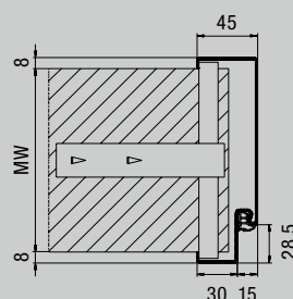
Profile 21101
