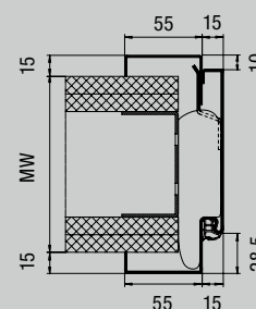
Profile 31103, rebated
