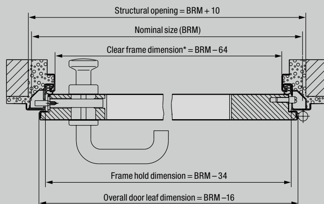
Fitting versions
