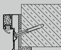
Diagonal fixing (Unplastered brickwork / concrete)
