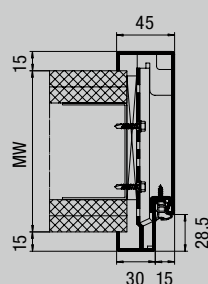
Profile 21180, rebated
