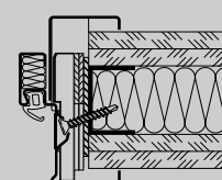
Diagonal fixing (Gas concrete)
