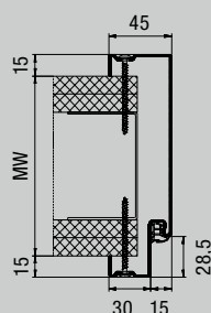
Profile 21120, screw fixing through frame face
