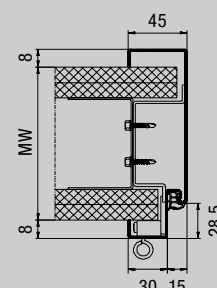
Profile 21120
