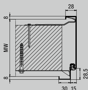
Profile 21100
