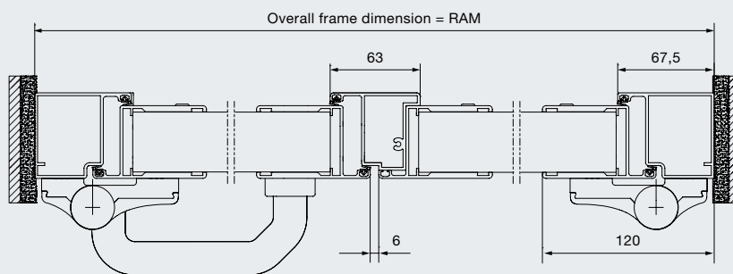
Horizontal view
