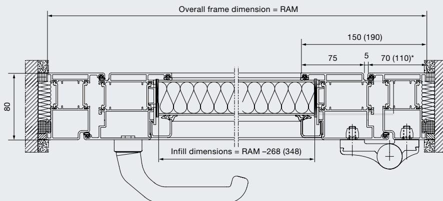
Horizontal view
