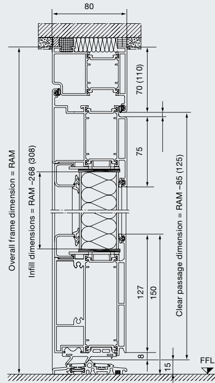
Vertical view
