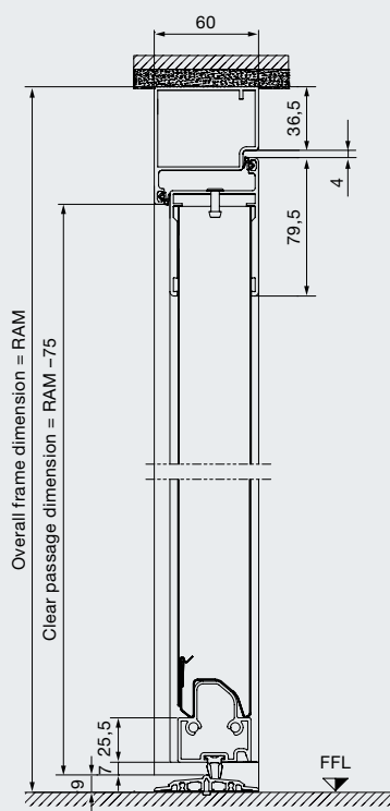
Vertical view
