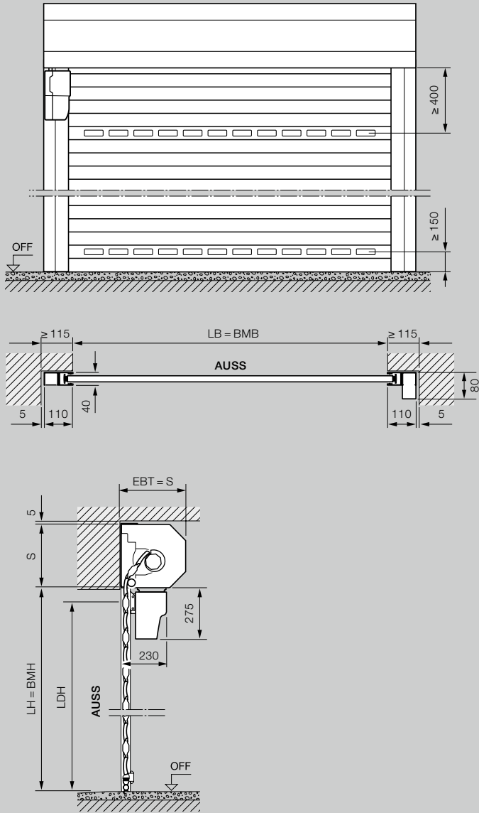
Size range for internal and external roller garage doors
