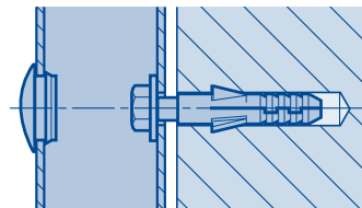
Screw fixing through the frame
