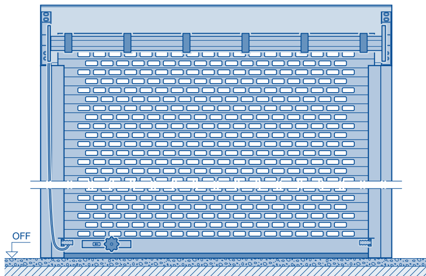
Pull cord viewed from inside, left
