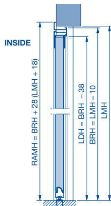
Internal fitting
