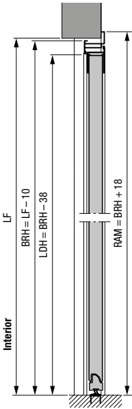
Side door with aluminium corner frame, profile type 2 External fitting
