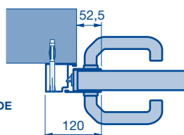
Profile type 2
