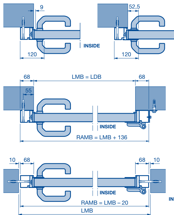
Profile type 1
