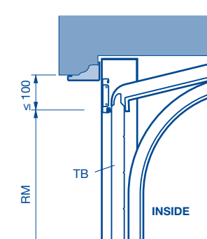
Angle section
