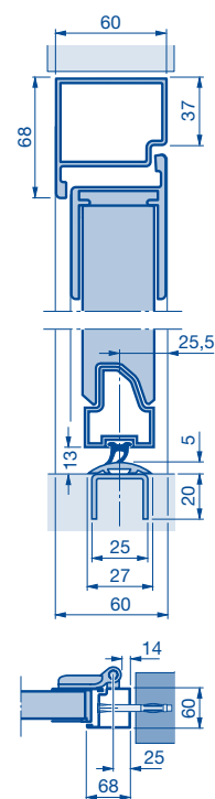
Profile type 1 / 2
