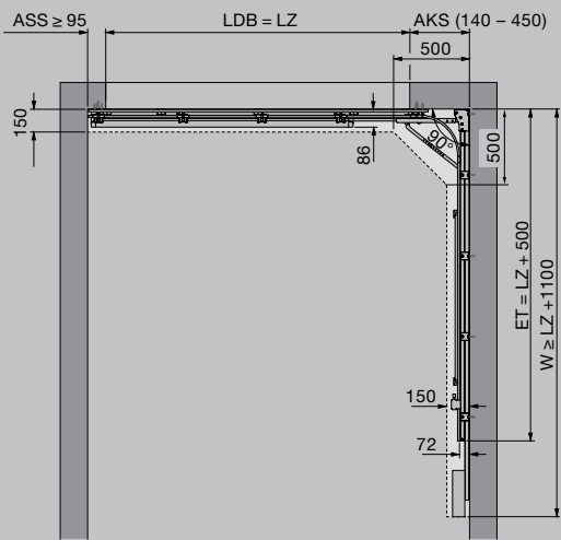
Track application DS (double track, operator wall fitting)
