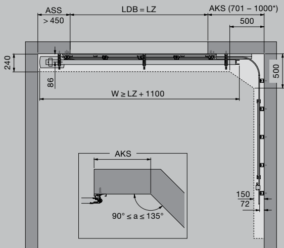
Track application ES (single track, operator ceiling fitting B)
