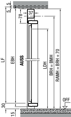
Vertical view Door without threshold
