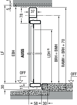
Vertical view Door with threshold
