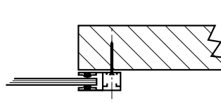
Fitted to existing or New Timber Frame
