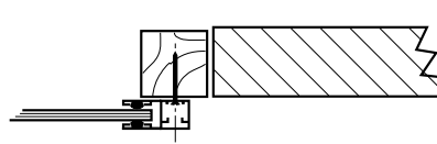
Fitted to existing or New Timber Frame
