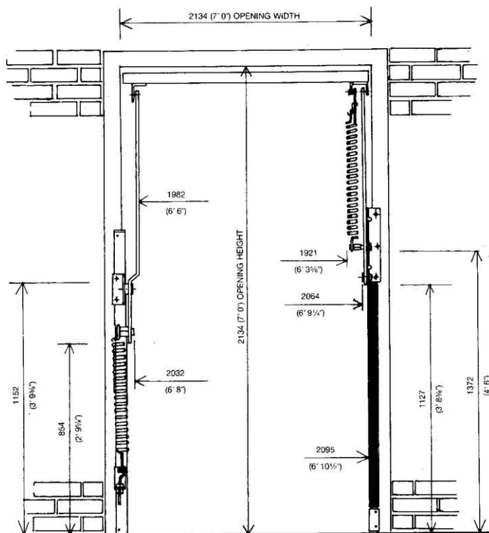
standard retractable gear CD150,200,250
