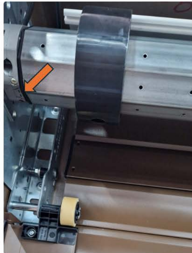
Operator with mechanical end position adjustment
